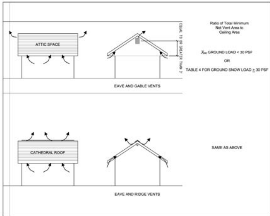
Figure 8 - Roof Ventilation Configurations
